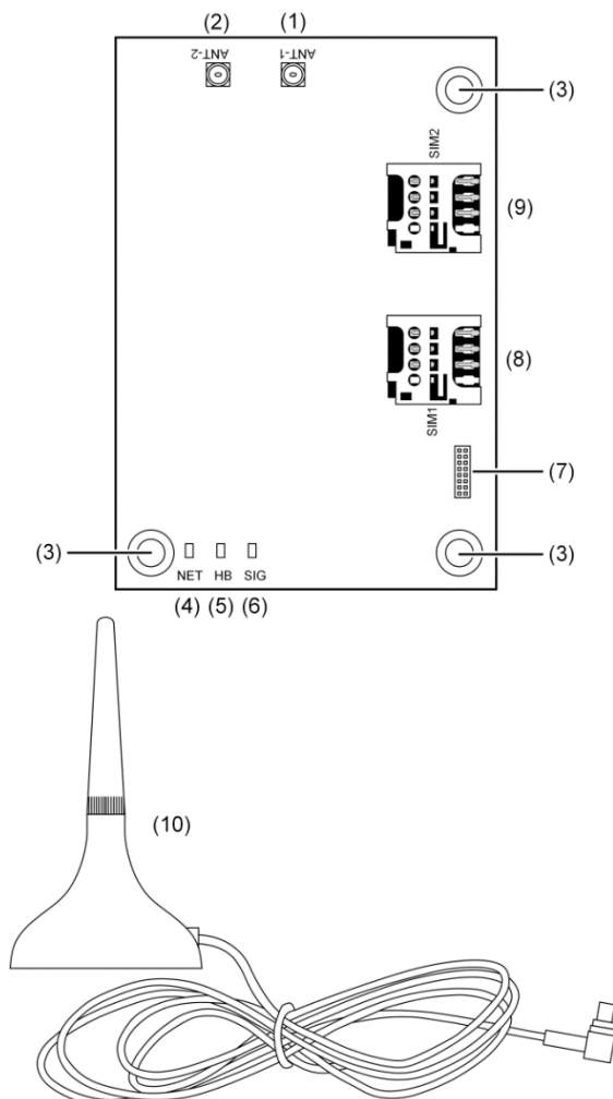
Figure 1: TS1054 module details
